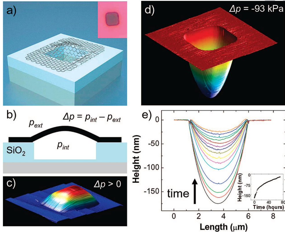
Figure 2. (a) Schematic of a graphene sealed microchamber. (Inset) optical image of a single atomic layer graphene drumhead on 440 nm of SiO 2 . The dimensions of the microchamber are 4.75 \mu\text{m} \times 4.75 \mu\text{m} \times 380 \text{nm} . (b) Side view schematic of the graphene sealed microchamber. (c) Tapping mode atomic force microscope (AFM) image of a \sim 9 \text{nm} thick many layer graphene drumhead with \Delta p > 0 . The dimensions of the square microchamber are 4.75 \mu\text{m} \times 4.75 \mu\text{m} . The upward deflection at the center of the membrane is 90 nm. (d) AFM image of the graphene sealed microchamber of Figure 1a with \Delta p = -93 \text{kPa} across it. The minimum dip in the z direction is 175 nm. (e) AFM line traces taken through the center of the graphene membrane of (a). The images were taken continuously over a span of 71.3 h and in ambient conditions. (Inset) deflection at the center of the graphene membrane vs time. The first deflection measurement ( z = 175 \text{nm} ) is taken 40 min after removing the microchamber from vacuum. From Reference [4].
