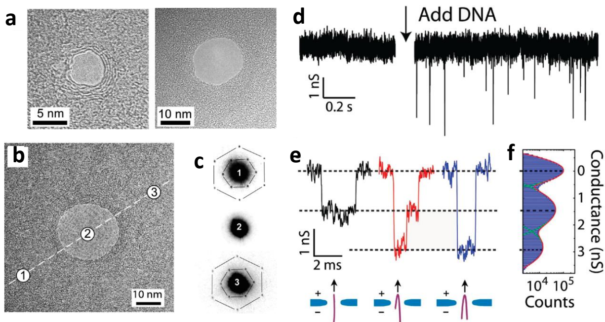
FIGURE 7. (a) Transmission electron microscopy (TEM) of nanopores drilled into multilayer graphene (b) TEM image of a 22 nm diameter pore in monolayer graphene. Incrusted numbers indicate spots where the diffraction patterns were recorded. (c) Diffraction patterns measured across the monolayer nanopore of panel left-b. (d-f) DNA translocation through a nanopore in a graphene monolayer. (d) Translocation of 48 kbp double-stranded \lambda -DNA across a 22 nm nanopore within a graphene monolayer, showing the baseline conductance and blockade events upon addition of DNA. (e) Examples of translocation events of nonfolded (black), partially folded (red), and fully folded (blue) DNA molecules recorded at 200 mV in the 22 nm pore. (f) Conductance histogram collected from 1222 translocation events, including the open-pore conductance before and after the event. Adapted from reference [3].
