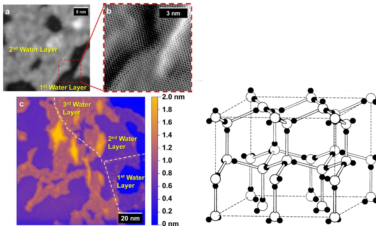
Figure 5. Scanning tunneling microscopy topographic scans of few layered water confined between graphene and mica. (a) 30 nm by 30 nm image showing the first two water layers on the mica surface. (b) Zoomed-in spatial derivative of the boxed region in (a) showing the honeycomb lattice of the monolayer graphene coating. (c) 100 nm by 100 nm false-colored topographic image of graphene-water-mica system. Three layers of water are visible, as well as a graphene grain boundary, which is labeled by the dotted white line. The protrusions coming out of the third water layer could be due to either contaminants trapped under the graphene or to the water displaying increasing bulklike properties as it gets further from the mica surface. Scanning conditions are -0.35 V sample bias and 1 nA tunneling current. The right panel shows the lattice structure of ice crystal. Adapted from reference [5] and [8].
