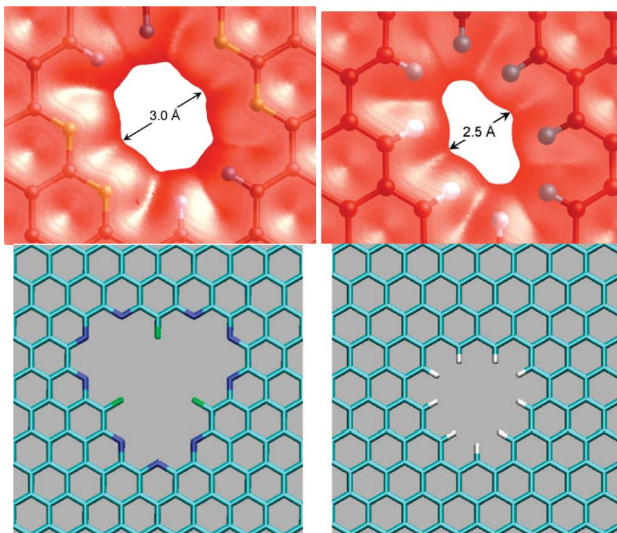
Figure 6: (Top) Pore electron density iso-surface of (left) nitrogen functionalized and (right) hydrogen-terminated porous graphene (isovalue of 0.02 \text{ e}/\text{\AA}^3 ). (Bottom) Functionalized graphene nanopores. (Left) The F-N-terminated nanopore. (Right) The H-terminated nanopore. Adapted from reference [1] and [6].
