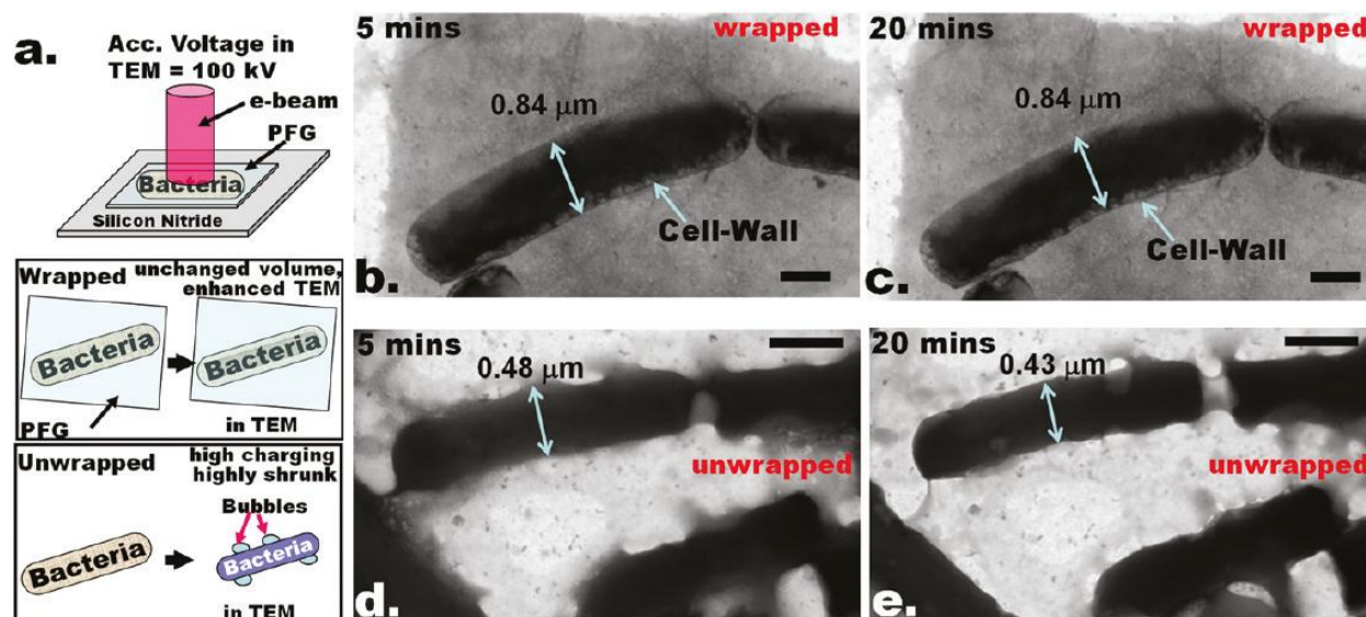
Figure 3: (a) Protein functionalized graphene (PFG) wrapping of bacteria prohibits shrinking under TEM. (b, c) Representative TEM images of wrapped bacterium (WB on 100 nm thick Si 3 N 4 windows) exhibits no shrinkage from the original size after 5 and 20 min exposure. (d, e) Representative unwrapped bacteria (UWB) exhibit ~75% shrinkage after only 5 min under TEM vacuum (minimum time to obtain micrograph). Extensive bubbling is also observed during imaging, attributed to boiling of the volatile component of the cell's intracellular region (see videos in Supporting Information). Scale bar = 500 nm. Note that under the same conditions, the cell wall of the wrapped bacteria is clearly discernible. This is attributed to significantly reduced charge accumulation due to the conductive PFGs (due to \pi electrons). Further, it has been shown that graphene[7] and graphene oxide[10, 11] can act as a great electron-transparent substrate for TEM imaging without the need for staining biological samples. From reference [12].
